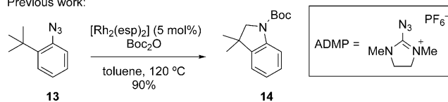
Scheme 3. Rhodium-catalyzed azide decomposition to form the indoline system. Reagents and conditions: a) ADMP (2 equiv), DMAP (3 equiv), MeCN, 50 °C, 3 h, 56%; b) [\text{Rh}_2(\text{esp})_2] (5 mol %), \text{Boc}_2\text{O} (1 equiv), toluene, 120 °C, 16 h, 29%. ADMP = 2-azido-1,3-dimethylimidazolinium hexafluorophosphate, DMAP = 4-dimethylaminopyridine, esp = \alpha,\alpha,\alpha',\alpha' -tetramethyl-1,3-benzenedipropionic acid, Boc = tert -butoxycarbonyl.
