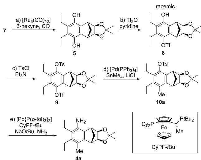
Scheme 2. Synthesis of aniline intermediate 4a toward herbindole B ( 1 ). Reagents and conditions: a) [\text{Ru}_3(\text{CO})_{12}] (4 mol %), 3-hexyne (1.1 equiv), CO (1200 psi), N -methylpiperidine, 160 °C, 2 days, 39%; b) \text{Tf}_2\text{O} (1.05 equiv), pyridine (1.2 equiv), \text{CH}_2\text{Cl}_2 , 0 \rightarrow 20 °C, 2 h, 58%; c) \text{TsCl} (1.1 equiv), \text{Et}_3\text{N} (3 equiv), \text{CH}_2\text{Cl}_2 , 0 \rightarrow 20 °C, 12 h, 93%; d) \text{SnMe}_4 (1.5 equiv), [\text{Pd}(\text{PPh}_3)_4] (10 mol %), \text{LiCl} (5 equiv), DMF, 150 °C (microwave), 6 h, 91%; e) [\text{Pd}\{\text{P}(\text{o-tol})_3\}_2] (3 mol %), \text{CyPF-tBu} (3 mol %), \text{NaOtBu} (1.0 equiv), \text{NH}_3 (4 equiv), 1,4-dioxane, 100 °C, 22 h, 54%. Tf = trifluoromethanesulfonyl, Ts = tosyl, DMF = N,N -dimethylformamide, tol = tolyl.
