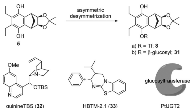
Scheme 8. Reagents and catalysts tested in the enantioselective triflation and diastereoselective glucosylation of meso -hydroquinone 5 . Reagents and conditions: a) \text{TiF}_2\text{O} (1.1 equiv), HBTM-2.1 (2.1 equiv), \text{CH}_2\text{Cl}_2 , -78 \rightarrow -40^\circ\text{C} , 1.5 days, 42% (63% ee ); b) PtUGT2 glucosyltransferase (0.034 mol%), DMSO, aqueous buffer, 20^\circ\text{C} , 5 days, 58% (d.r. 20:1).
